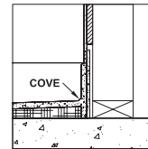
COVED DETAIL COVE OPTION # 2 ½" WALLS
