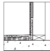
WALL DETAIL STRAIGHT WALL ¼" OR ½" WALLS
