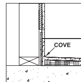
COVED DETAIL COVE OPTION # 3 ½" WALLS
