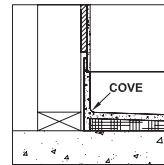
COVED DETAIL COVE OPTION # 1 ¼" WALLS
