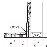
COVED DETAIL COVE OPTION # 4 ½" WALLS
