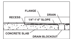
NO EGRESS THRESHOLD OPTION
