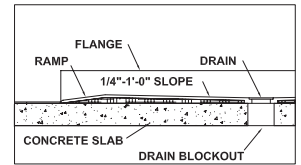
LOW EGRESS THRESHOLD OPTION
