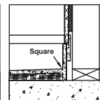
SQUARE WALL OPTION #4 1/2" WALLS
