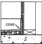
COVED WALL OPTION #2 1/2" WALLS
