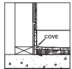
COVED WALL OPTION #1 1/2" WALLS
