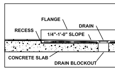
NO EGRESS THRESHOLD OPTION
