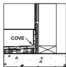
COVED DETAIL COVE OPTION # 2 1/2" WALLS
