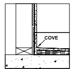
COVED DETAIL COVE OPTION # 3 1/2" WALLS
