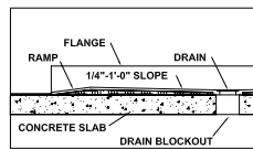
LOW EGRESS THRESHOLD OPTION
