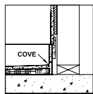
COVED DETAIL COVE OPTION # 4 1/2" WALLS
